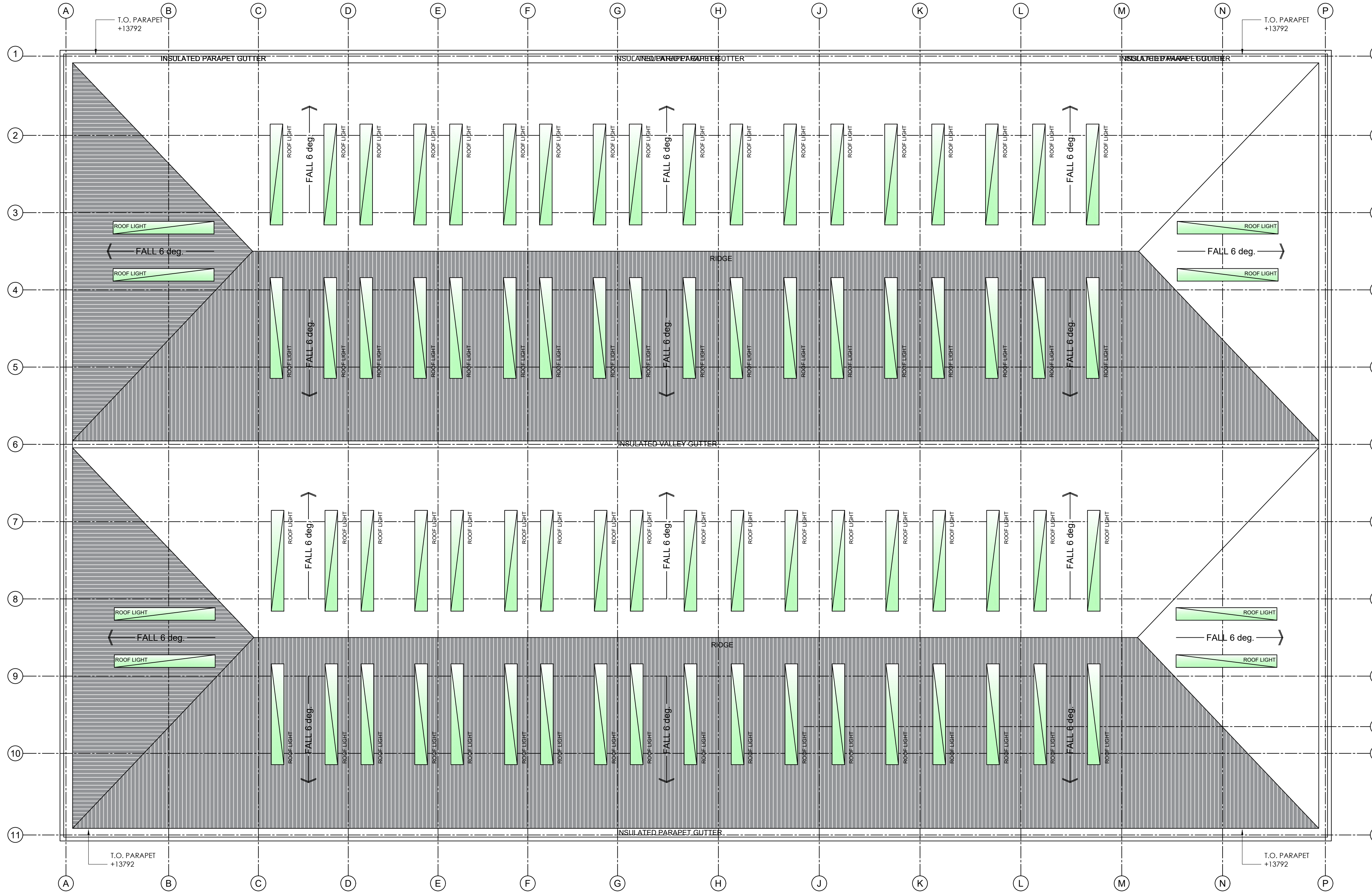
ROOF PLAN
