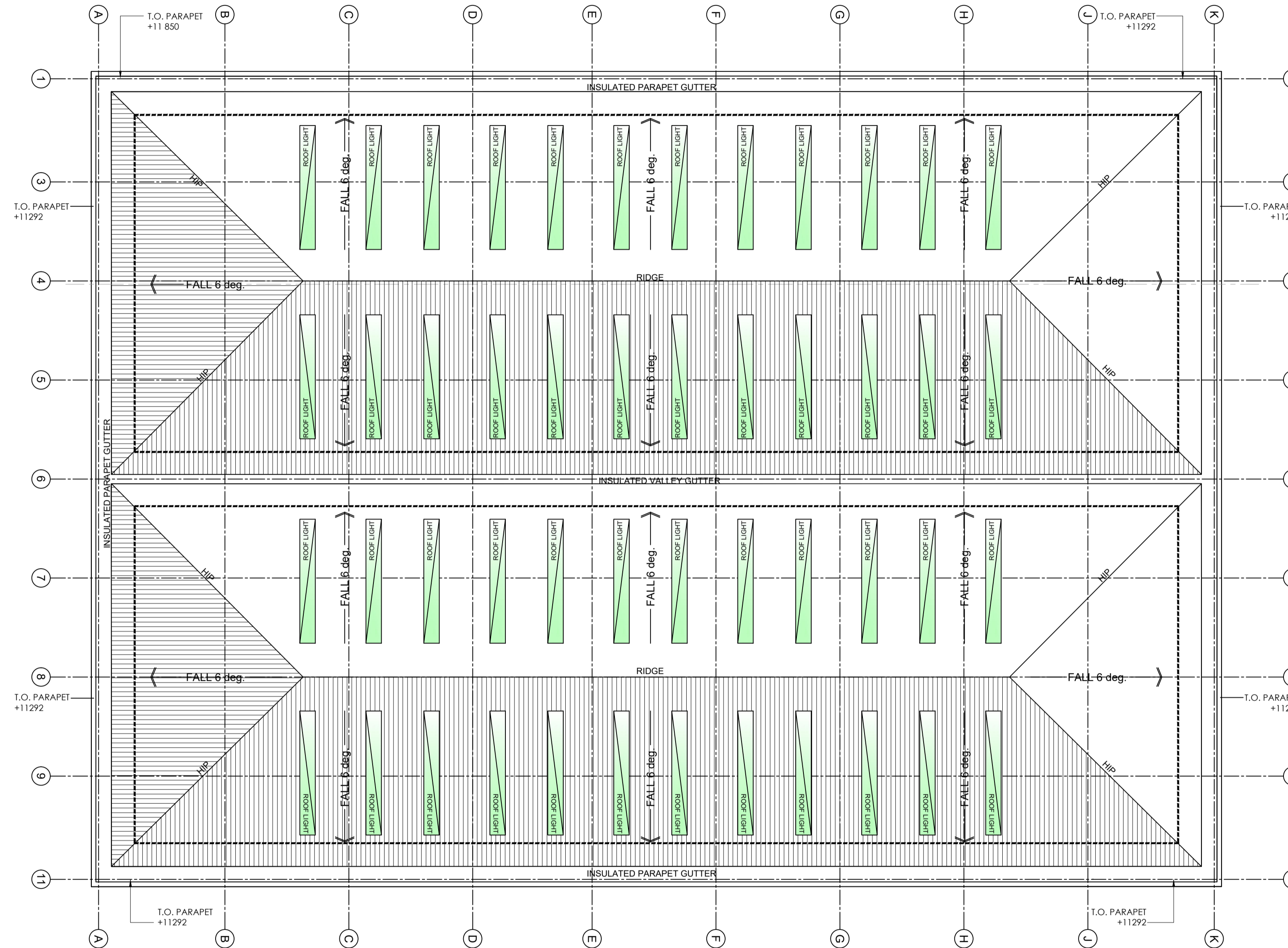
ROOF PLAN
